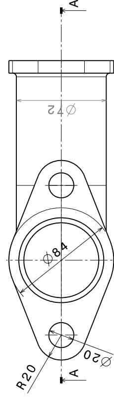
Front view Scale: 1:2
