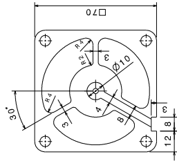
Auxiliary view C Scale: 1:1
